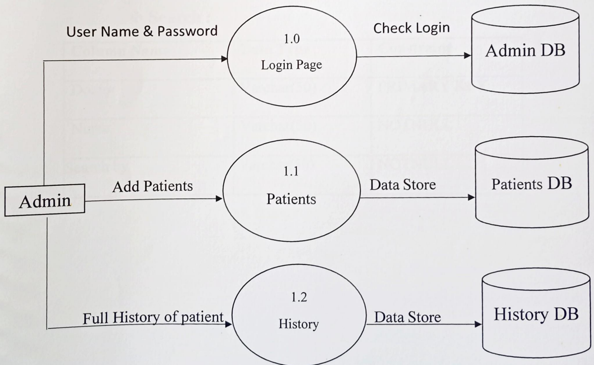
(Fig. 2.4.2) 1 st Level of DFD
